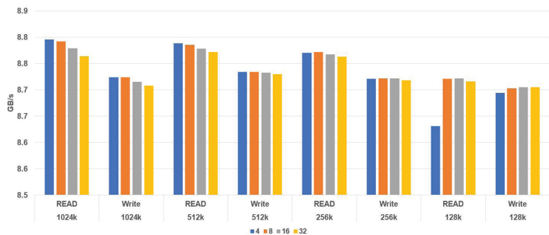
ATTO ExpressSAS 1280 GT Adapter Performance One JBOF, One Expander, 16 Drives
