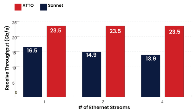
Ethernet NIC Receive & Send Performance
